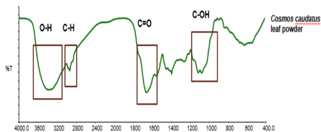
Fig. 2 FTIR spectrum of Cosmos Caudatus leaf extract
