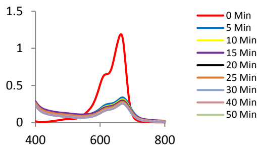
Fig. 7 Decolourisation of methyl blue in the presence of (3 mL) Cosmos Caudatus leaf extract and (10 mg) catalyst.
